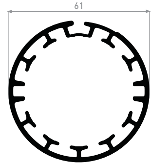
2 ad. / paket - 1.657 kg/m 2 pcs. / box - 1.657 kg/m
