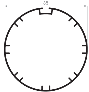
5 ad. / paket - 0.840 kg/m 5 pcs. / box - 0.840 kg/m
