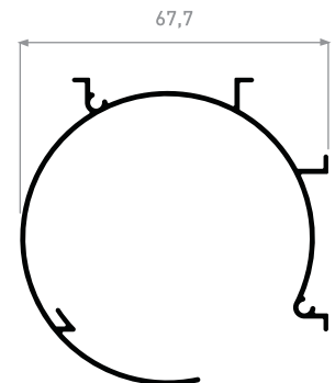
4 ad. / paket - 0.625 kg/m 4 pcs. / box - 0.625 kg/m
