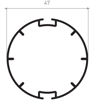
5 ad. / paket - 0.523 kg/m 5 pcs. / box - 0.523 kg/m
